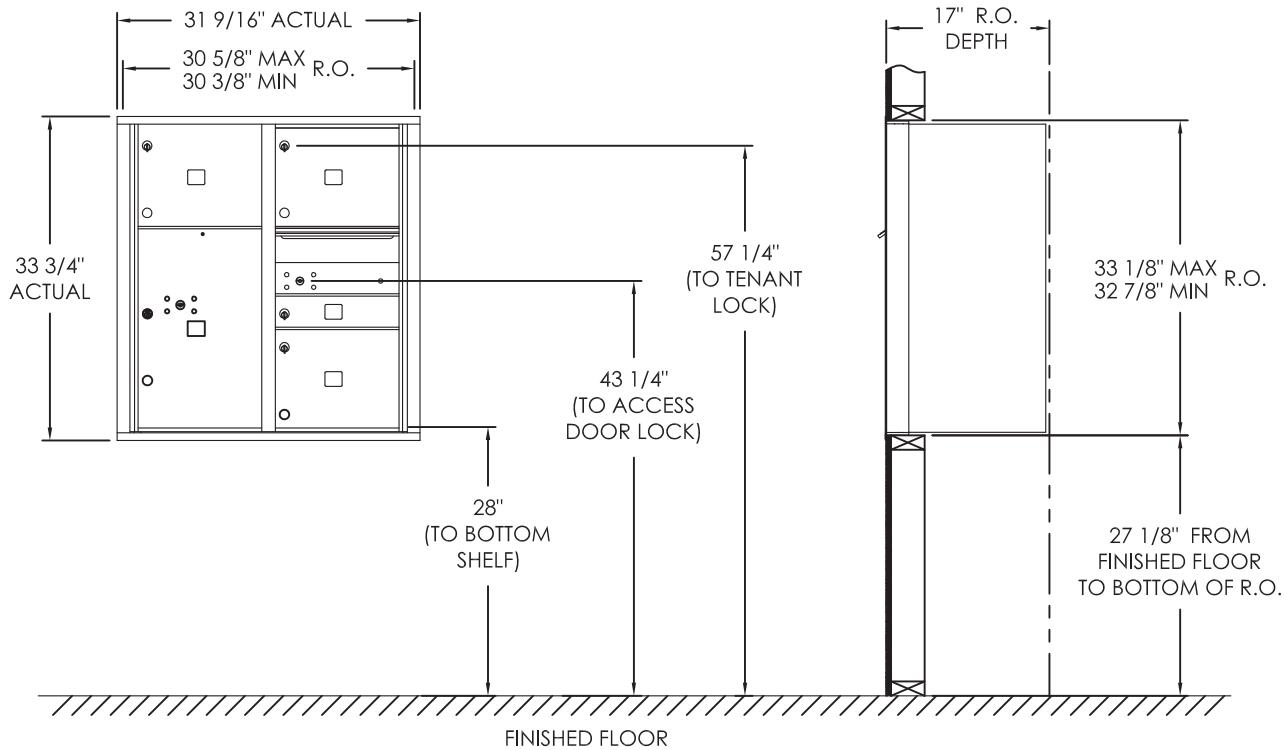
COMPARTMENT CHART
