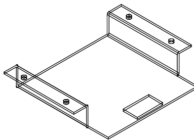
P/N 41703 LOCK SUPPORT BRACKET
