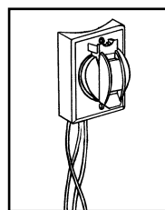
Post Electrical Outlet Item # CO-268 Curved to fit 3" O/D post. 1 1/4" hole required. 120 Volt only.
