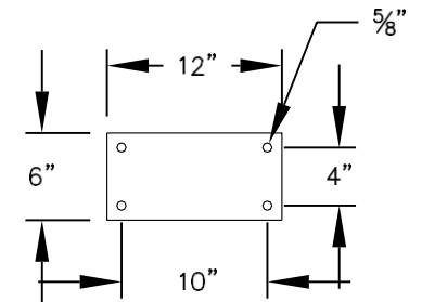
PEDESTAL TOP BOLT PATTERN
