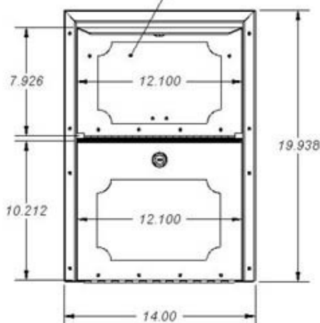
HOPPER ID DIMENSIONS 4.875 x 10.875
