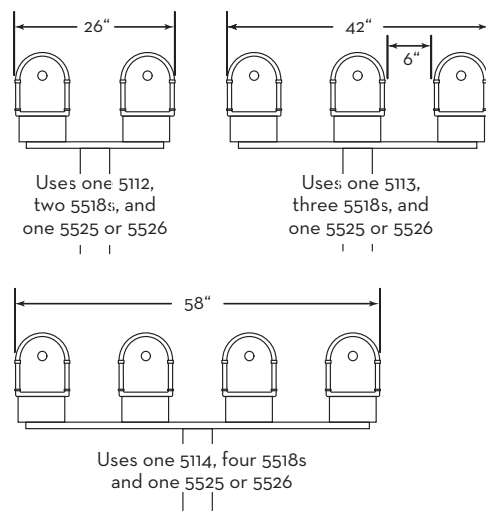
AVALON WITH STANDARD POST
