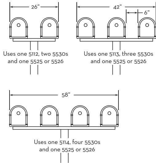
AVALON WITH STANDARD POST
