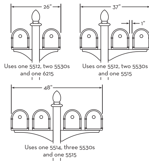
AVALON WITH DECORATIVE POST
