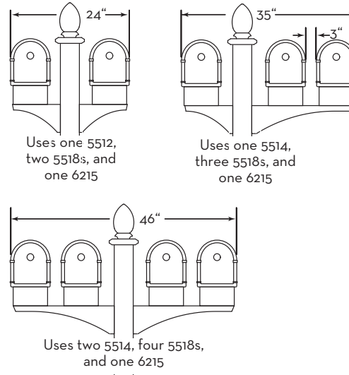
FAIRFIELD WITH DECORATIVE POST
