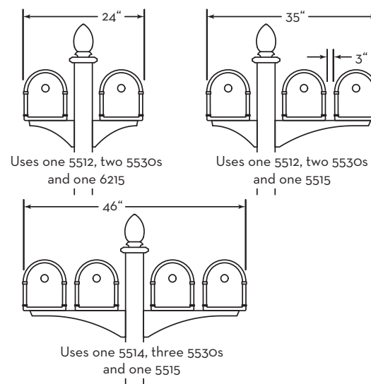
FAIRFIELD WITH DECORATIVE POST
