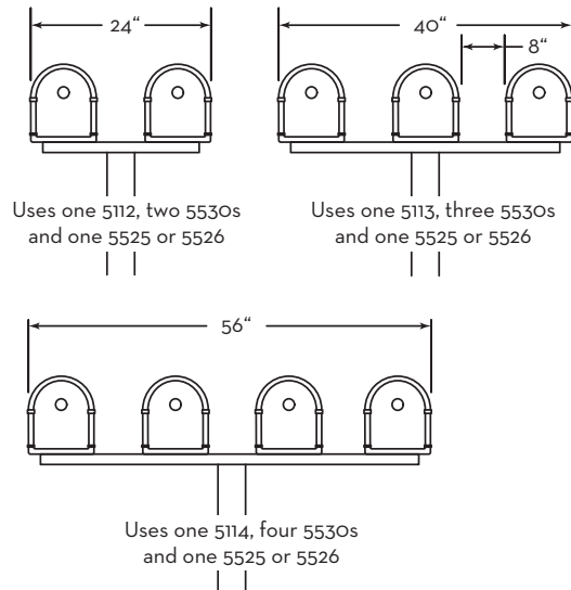
FAIRFIELD WITH STANDARD POST
