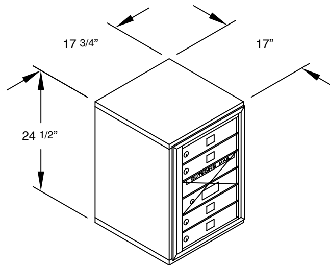
MODEL #3806S-04 - FRONT LOADING
