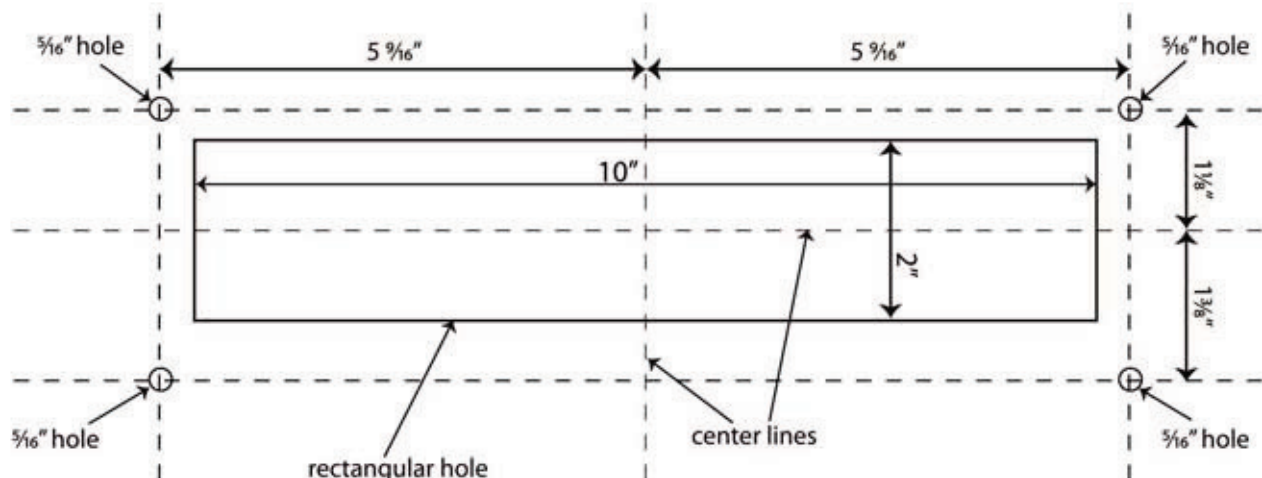
SMALL ( 11 \frac{1}{16}" \times 3 \frac{1}{4}" ) Mail Slot Installation Dimensions (do not scale)
