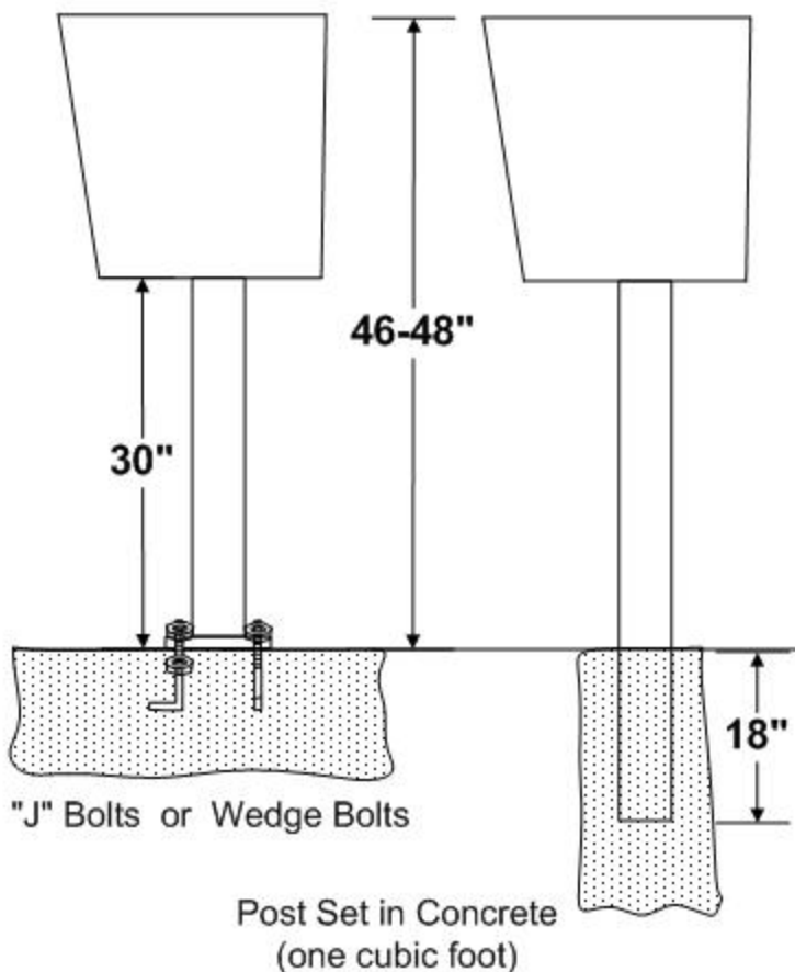
FIGURE C - Ground Installation
