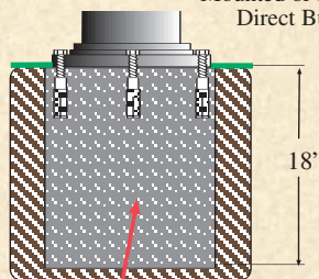
Cement Footer
