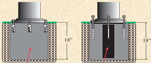
Cement Footer SPK-600 and SPK 606 Posts can be Surface Mounted or installed as Direct Burials
