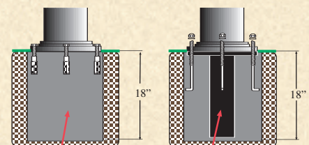
Cement Footer
