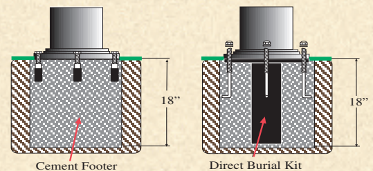
Cement Footer
