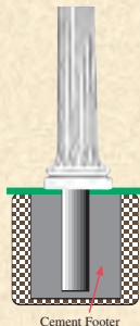
SPK-592, SPK-590 and SPK-678 posts require direct burial
