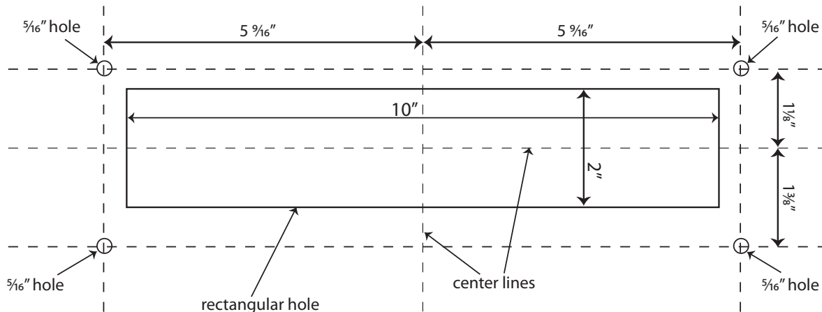
SMALL ( 11 \frac{1}{16} " x 3 \frac{3}{4} " ) Mail Slot Installation Dimensions (do not scale)
