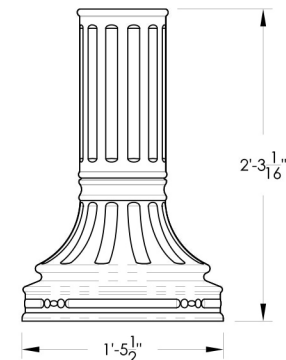
FRONT & SIDE VIEW TALL PEDESTAL (VOGUEPA28)
