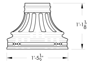
FRONT & SIDE VIEW SHORT PEDESTAL (VOGUEPA14)
