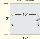
pedestal top bolt pattern
