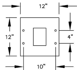
PEDESTAL BASE BOLT PATTERN
